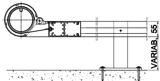
STAFFAGGIO - BRACKETS PATTES DE FIXATION
