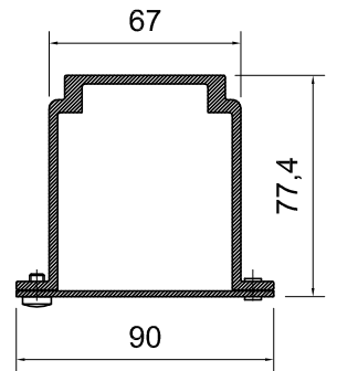
SUPPORTO CASSONETTO HEAD BOX SUPPORT SUPPORT CAISSON
